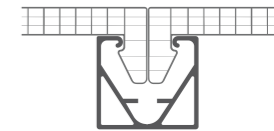
Reinforced AL profile
